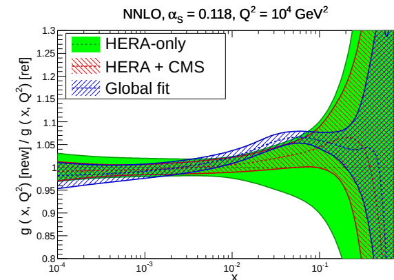
GLOBAL VS HERA+CMS: g & \bar{d}
