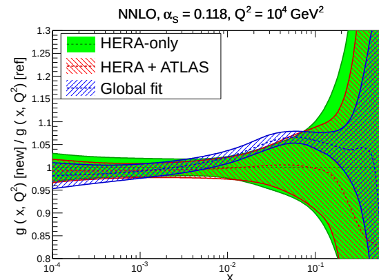
GLOBAL VS HERA+ATLAS: g & \bar{d}
