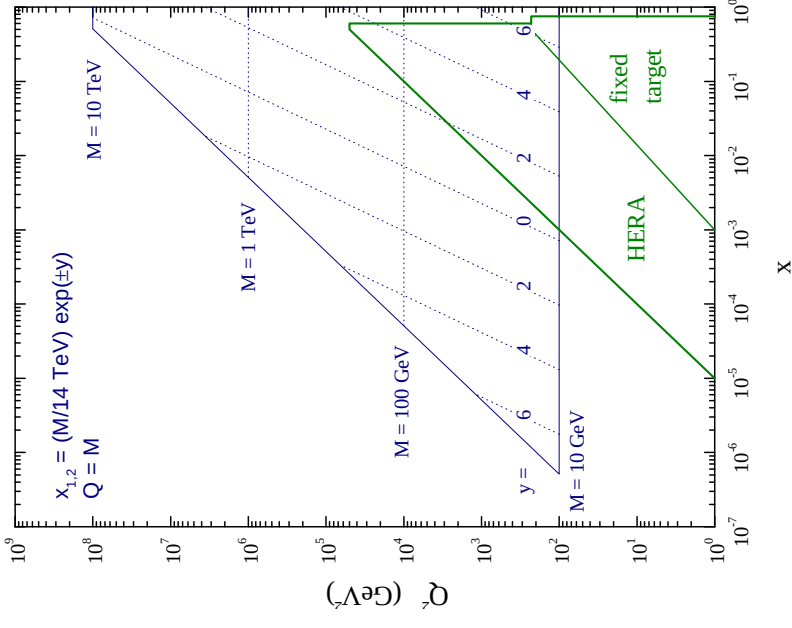
LHC parton kinematics
