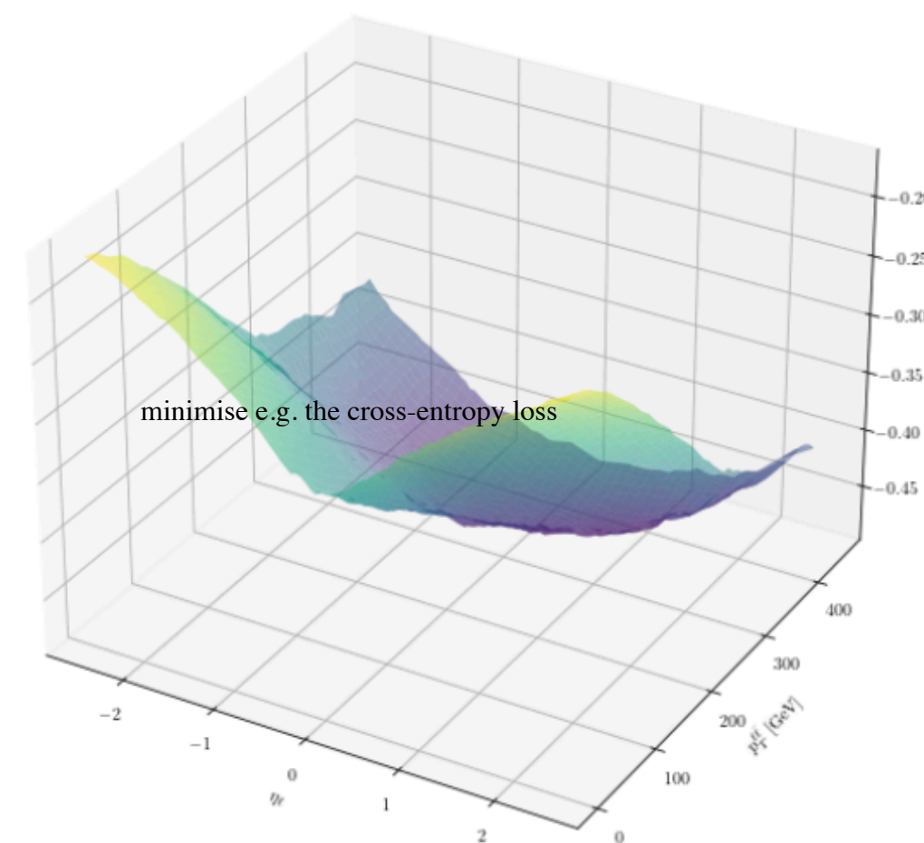
Unbinned, multivariate
