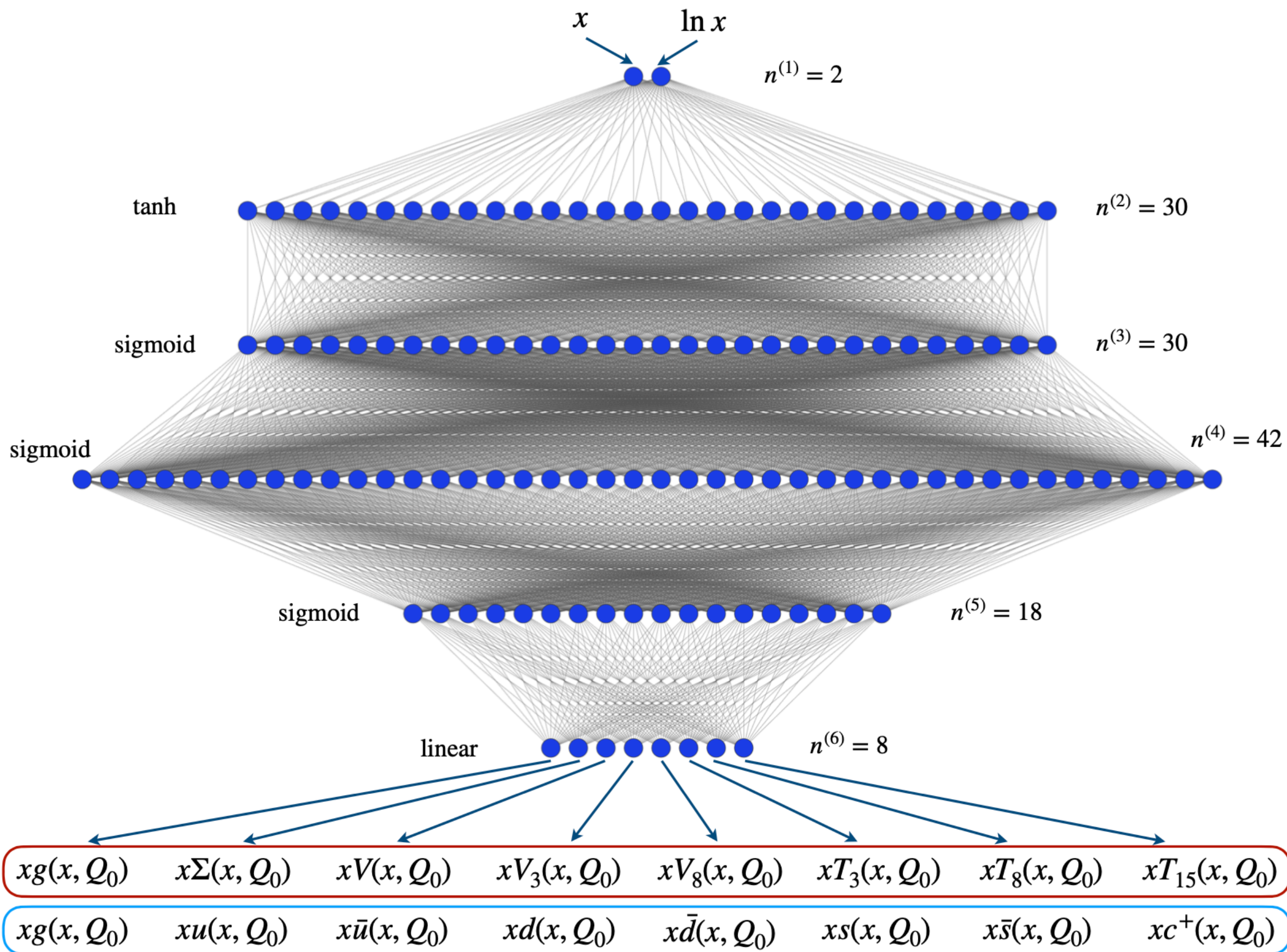
K-fold loss
