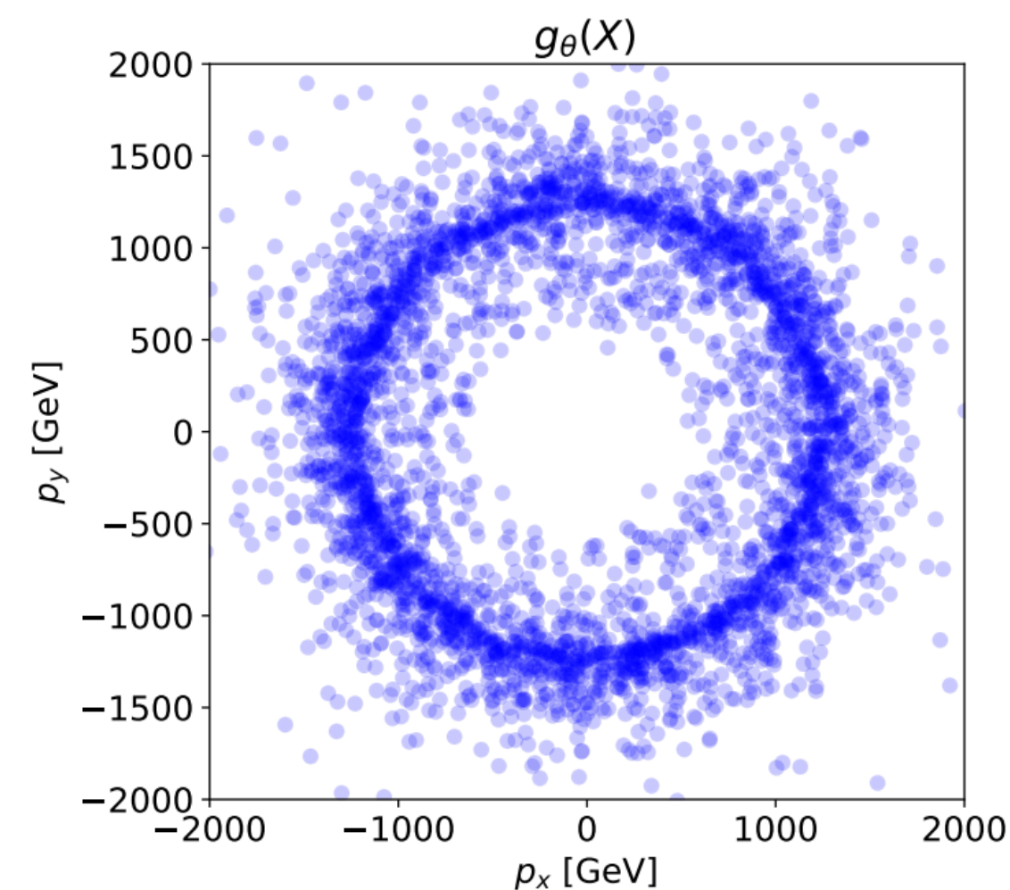
Symmetry GAN
