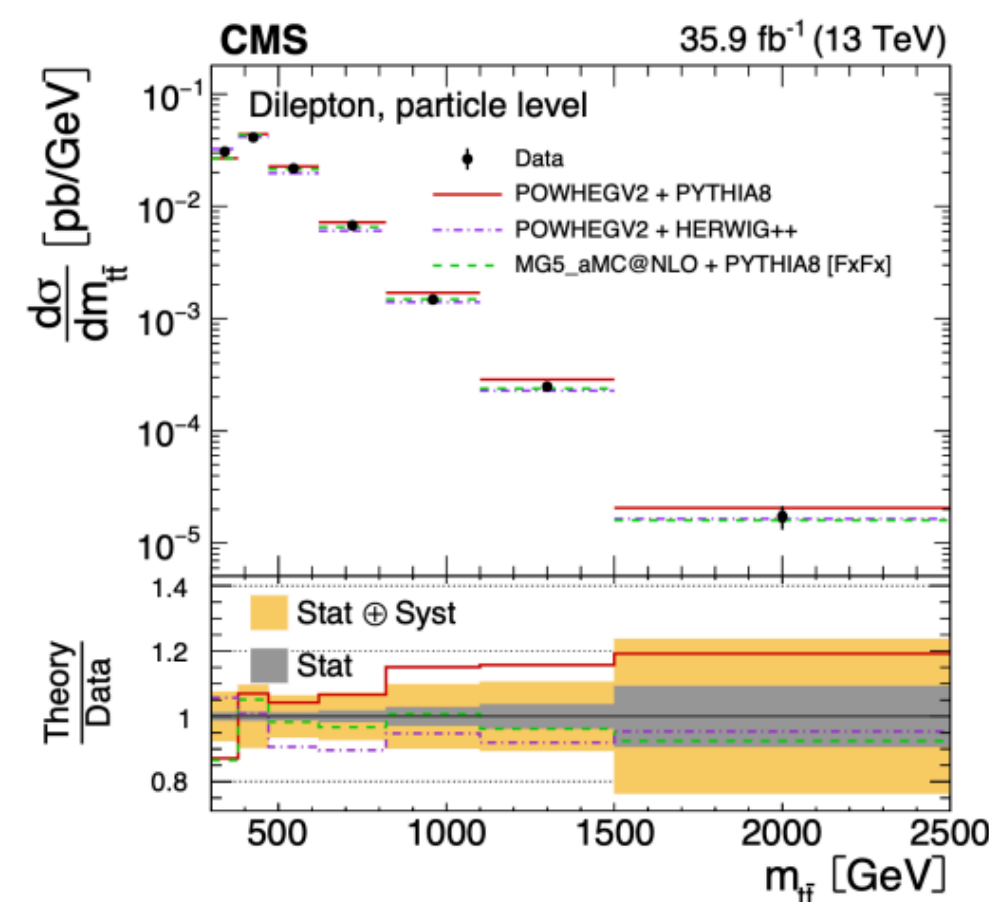
Binned, univariate
