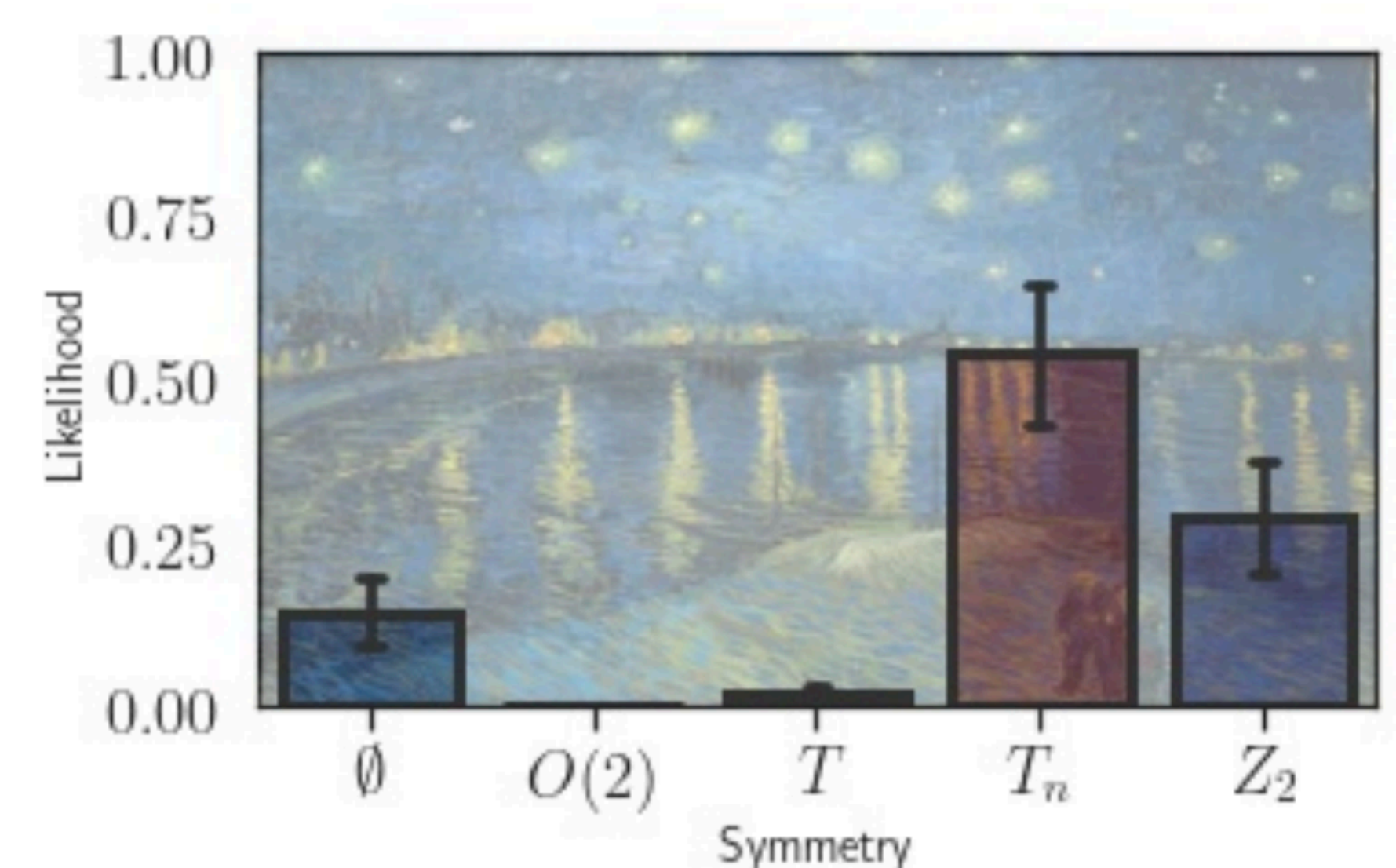
Classifiers
